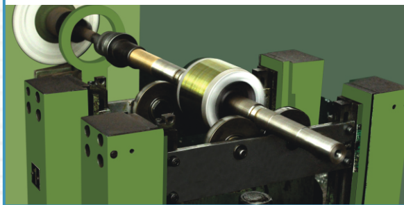
Rotor Balancing
