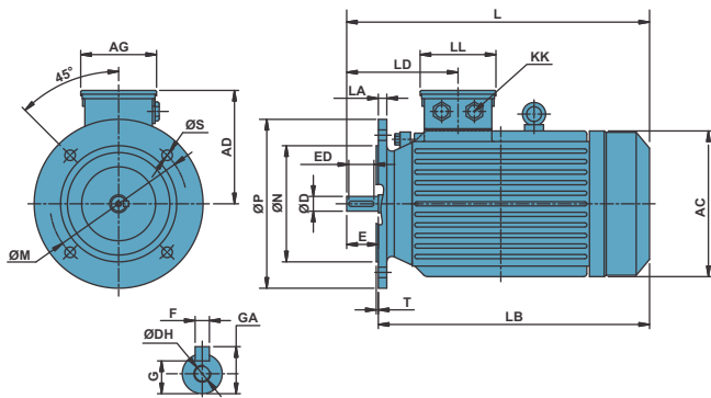
B5 Flange Mounted Motor
