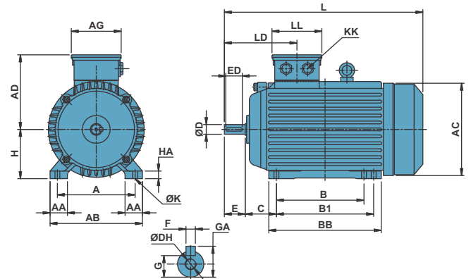
B3 Foot Mounted Motor
